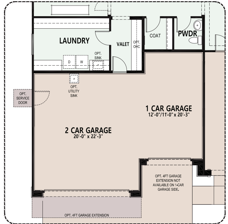
Opt. Expanded Laundry - Elevation D
