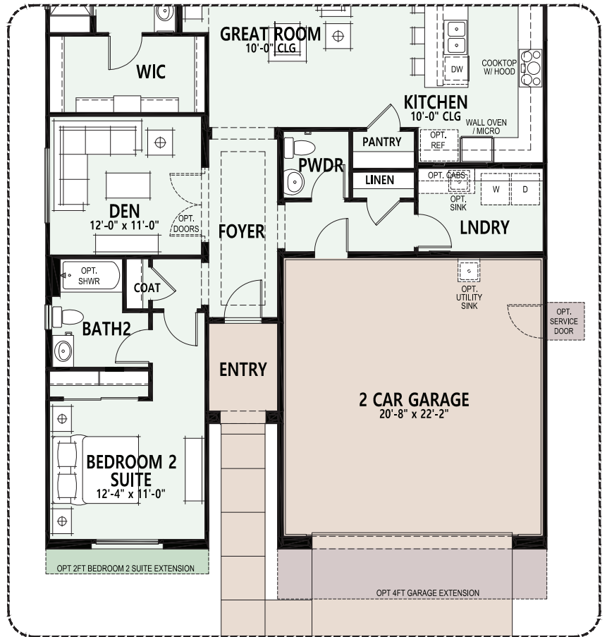
Alternate Built-in Kitchen w/ Opt. Powder Room
